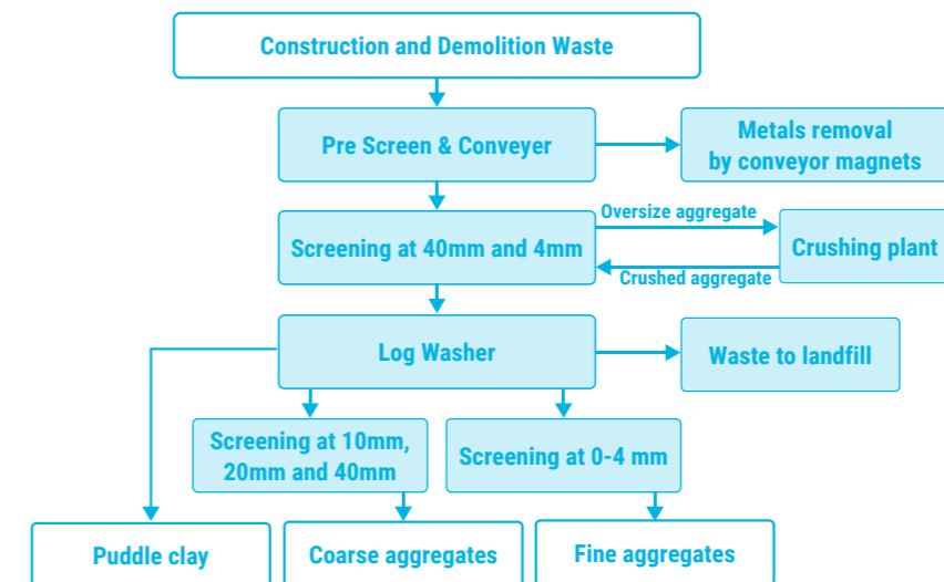
FIGURE 3-20 Process flow for the processing of CDW to extract building materials 51
