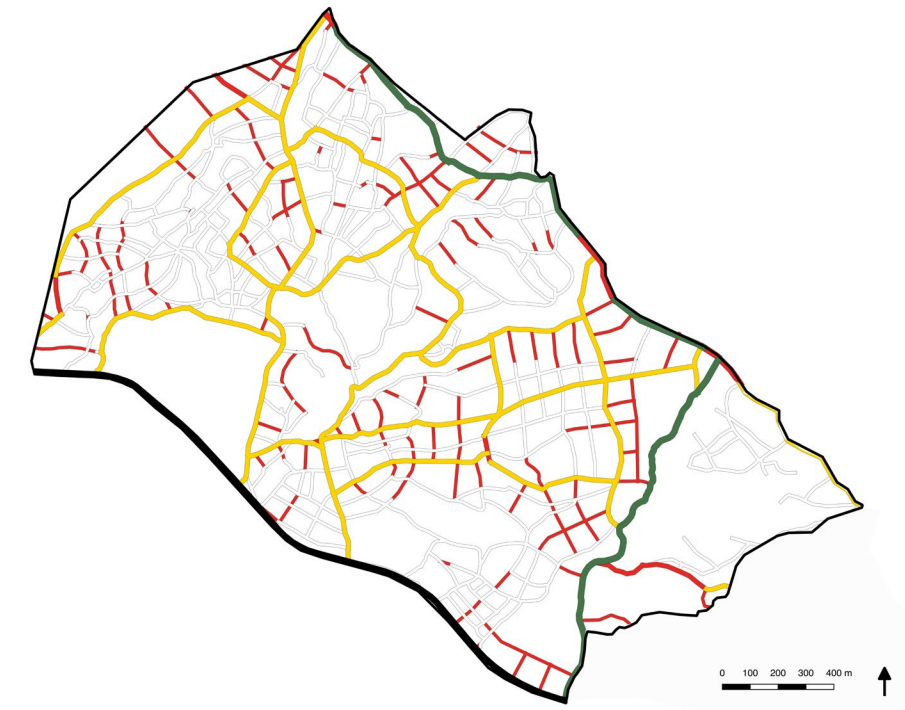
Fig.185: St.Christophe: Proposed street network
